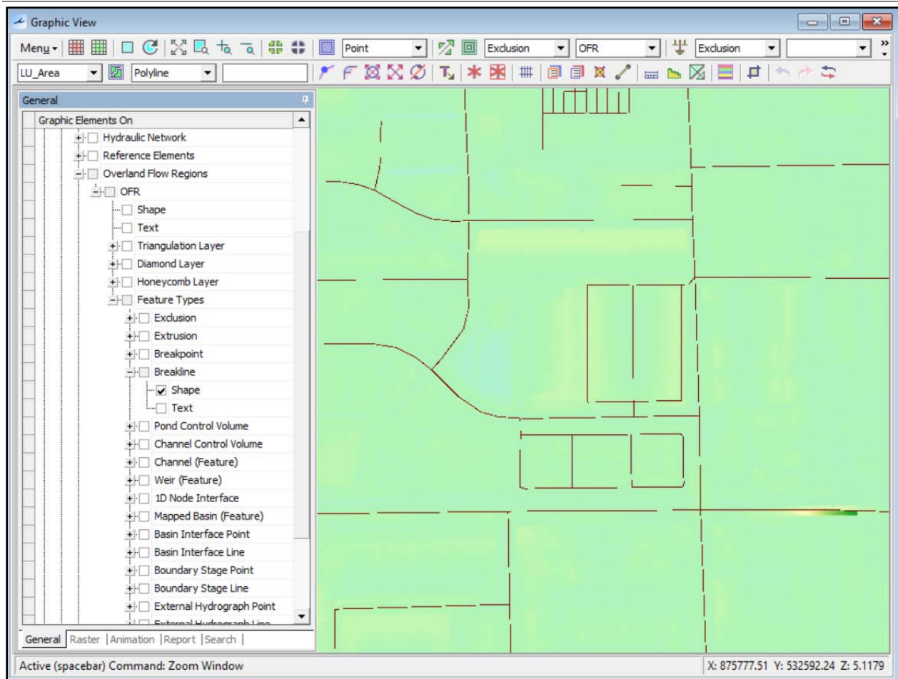
Figure 4-8 – Breakline Map Layer for a Section of the City’s Domain
