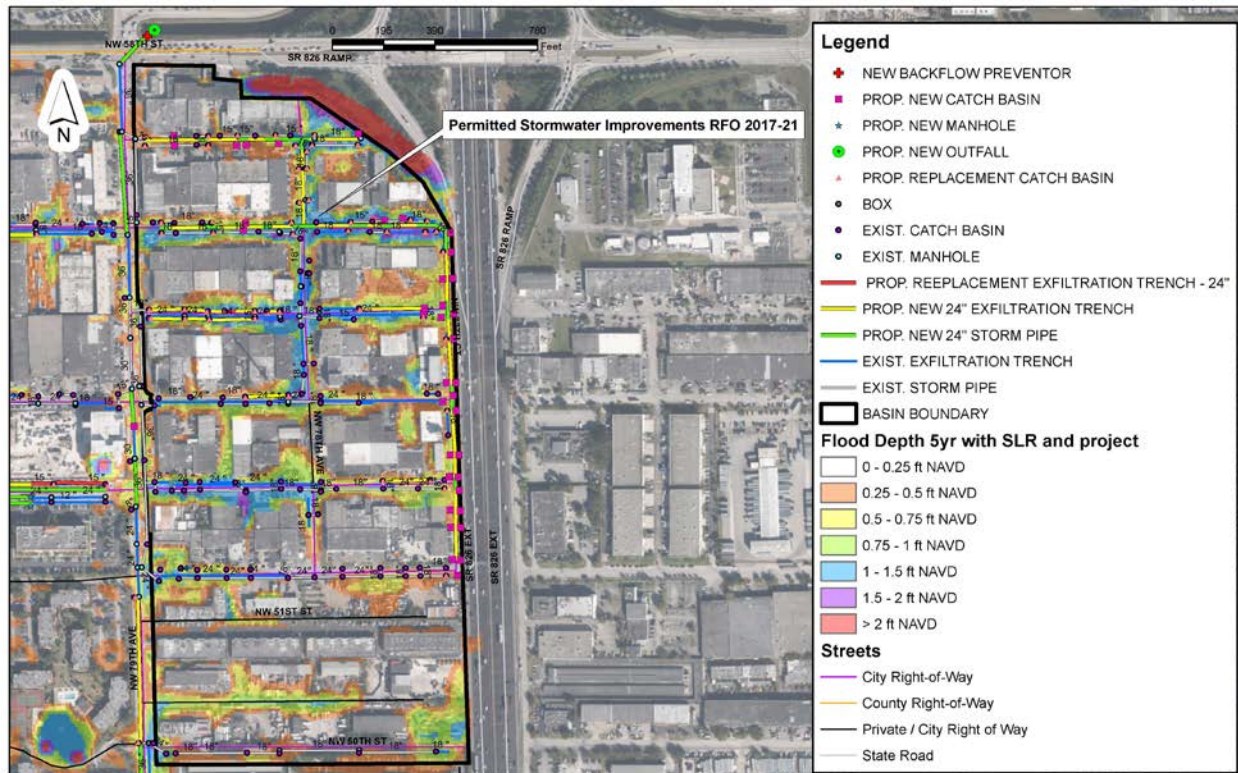
Figure 7-9 – Basin H-8 Proposed Outfall Location
