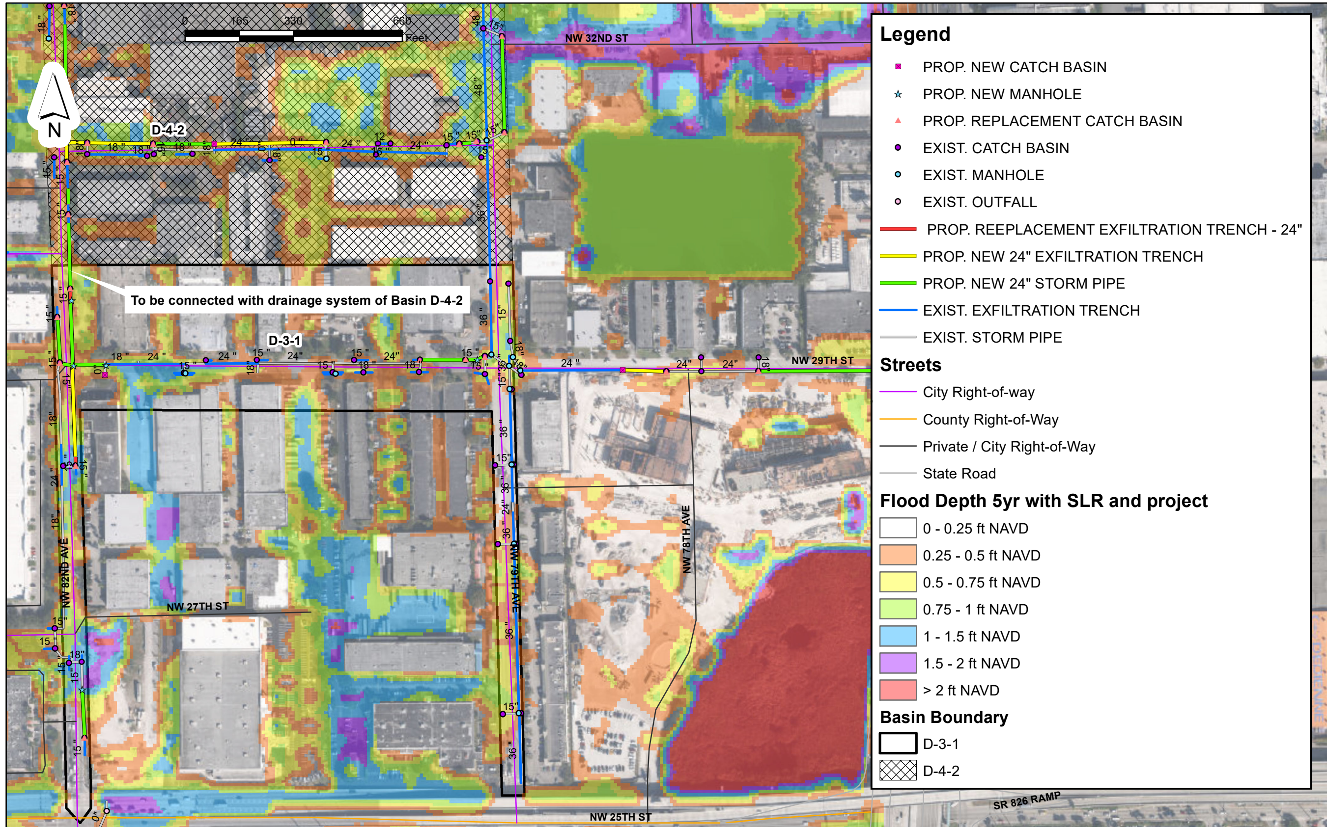
City of Doral Stormwater Management Master Plan Proposed Stormwater Projects Basin D-3-1 (Basin Rank 5) Cost Rank 6 - $421,231.74
