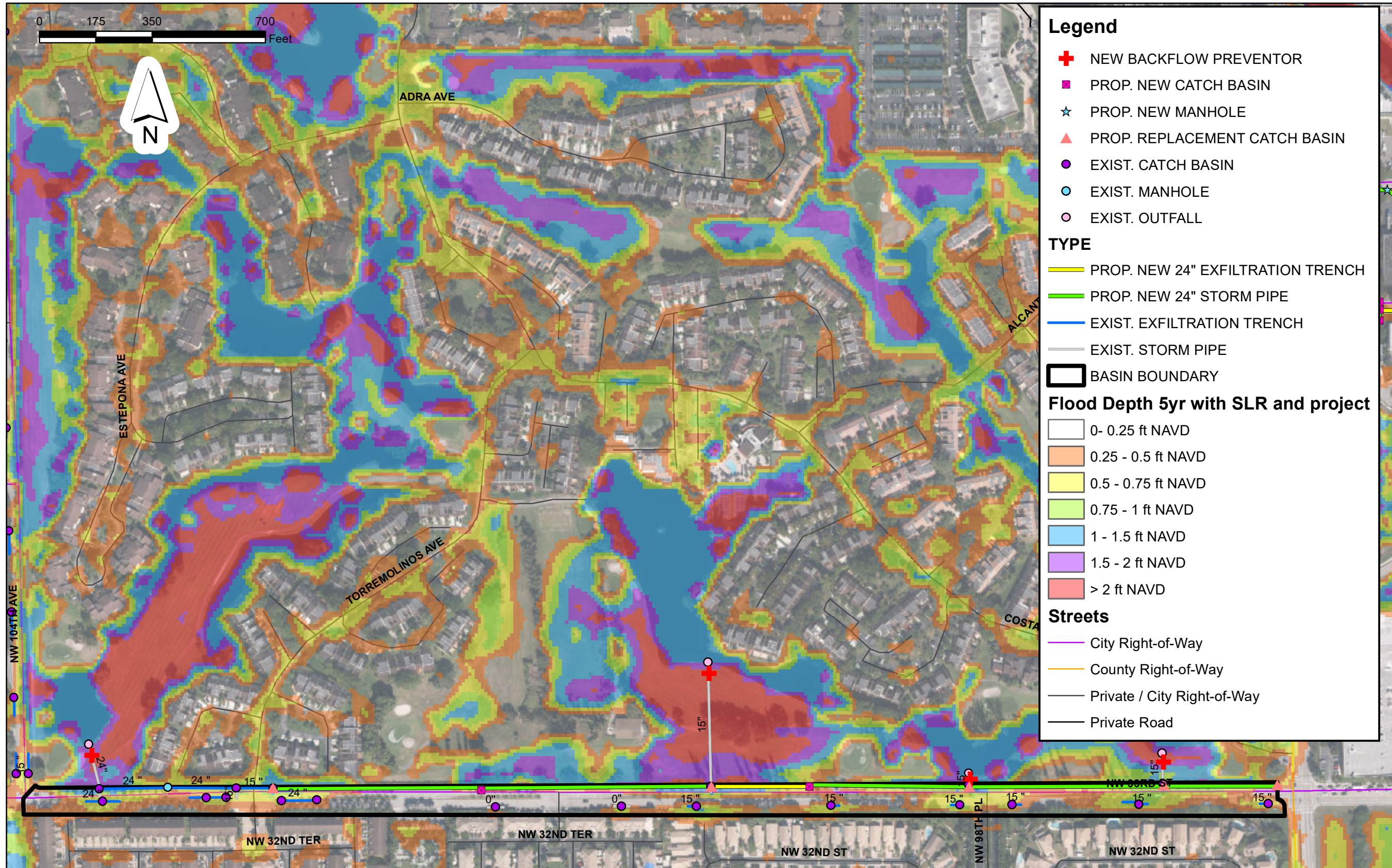
City of Doral Stormwater Management Master Plan Proposed Stormwater Projects Basin NW 33 ST (Basin Rank 7) Cost Rank 9 - $823,837.44
