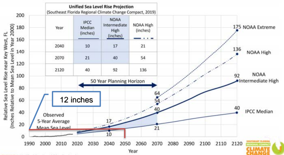
Figure 6-1 – Unified Sea Level Rise Projections for Southeast Florida (2019)
