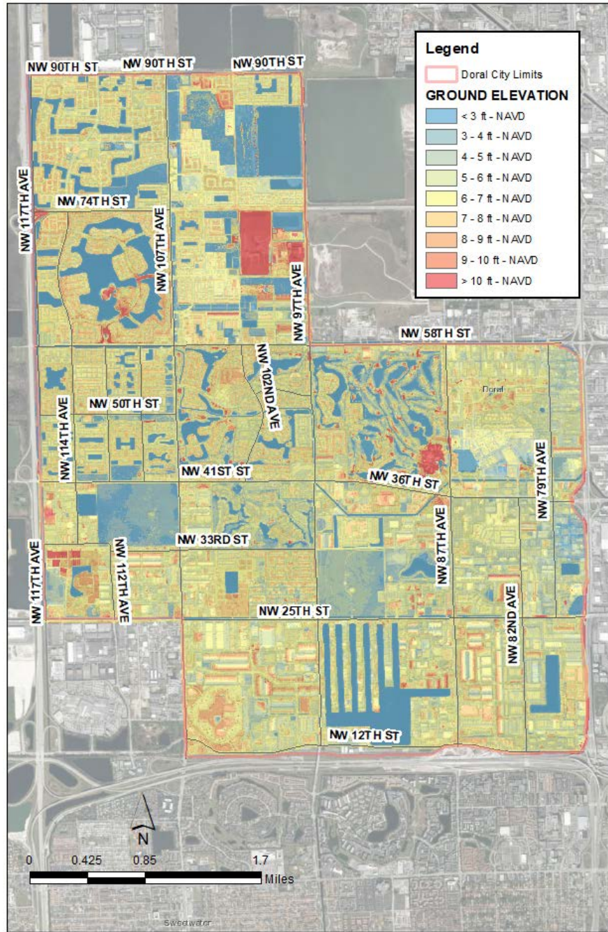
Figure 4-2 – City of Doral Topography
