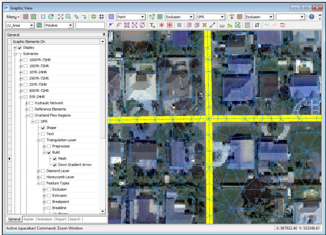
Figure 4-11 – Triangular Mesh and Breakline with Downgradient Arrows
