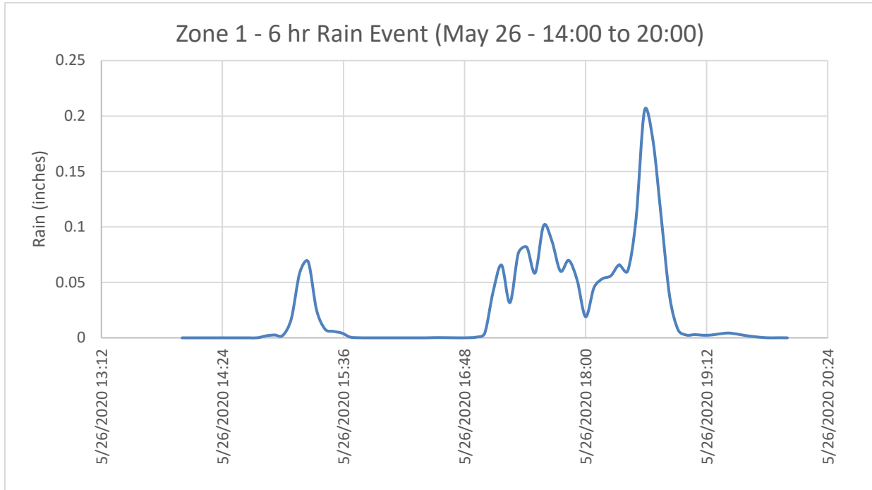
Figure 4-16 – Rain Zone 1 Hydrograph
