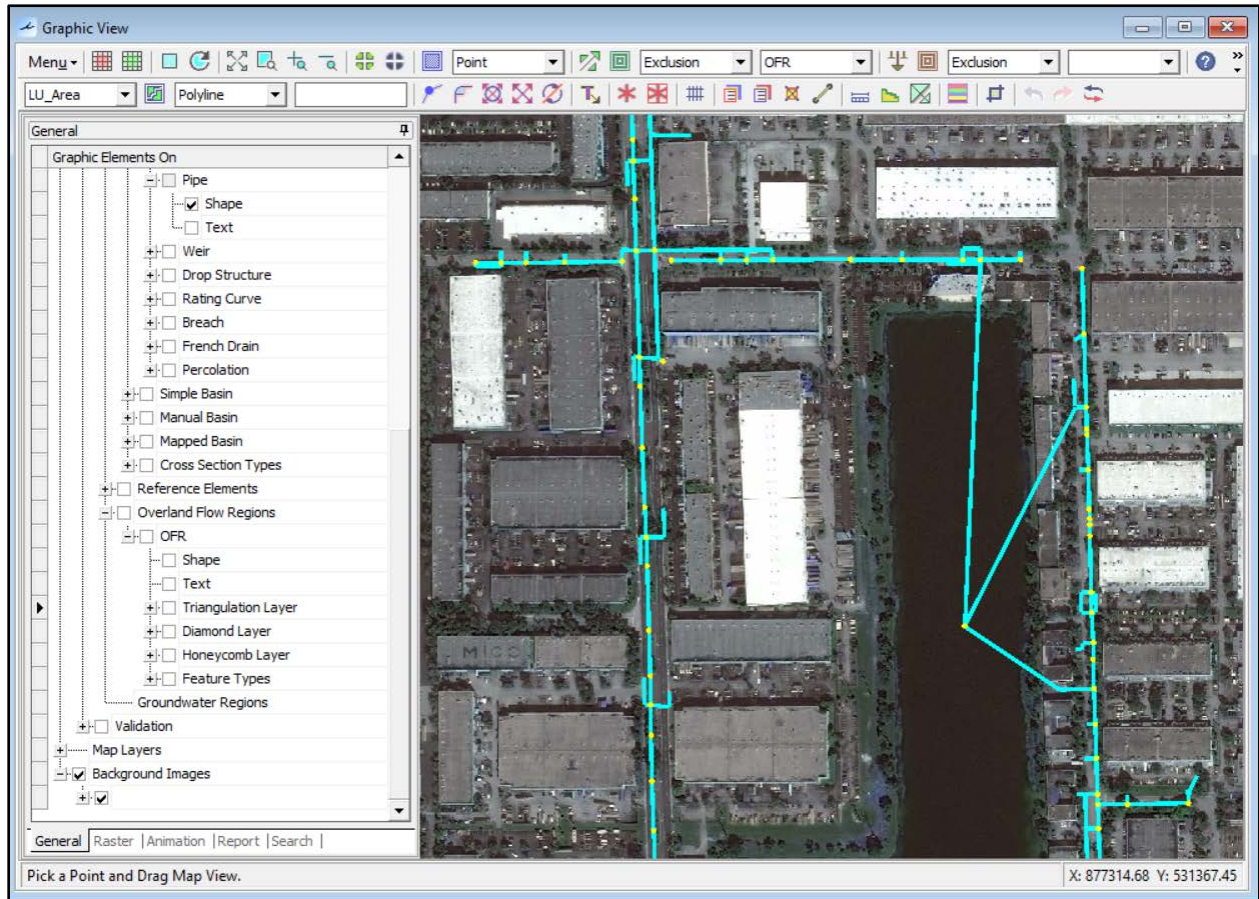
Figure 4-13 – Drainage Infrastructure within a Section of the City’s Domain
