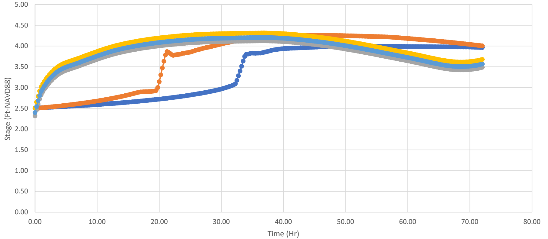
25YR-72HR TIME-STAGE HYDROGRAPH
