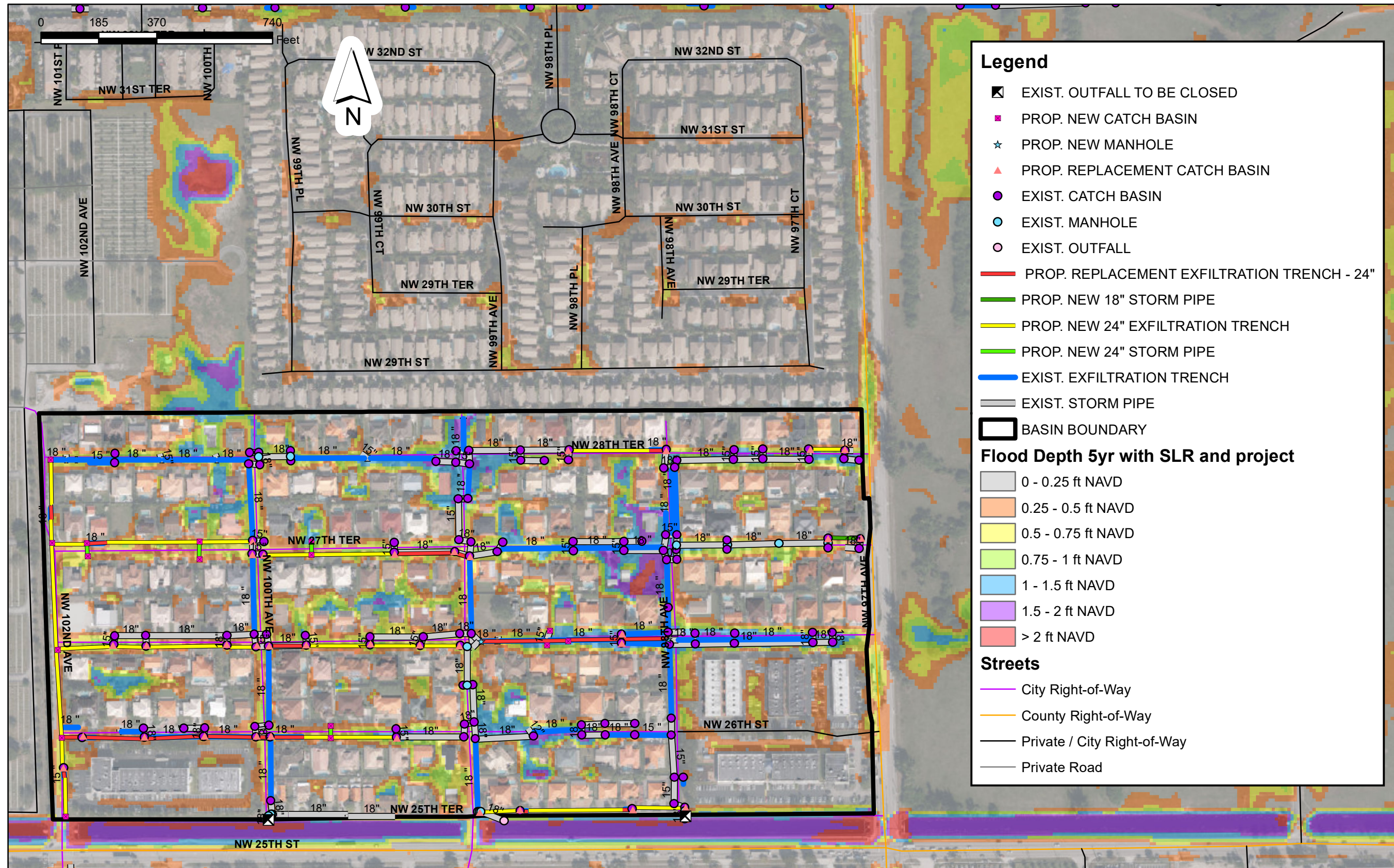
City of Doral Stormwater Management Master Plan Proposed Stormwater Projects Basin F1 no PS (Basin Ranking 2) Cost Effectiveness Rank 11 - $2,345,582.00
