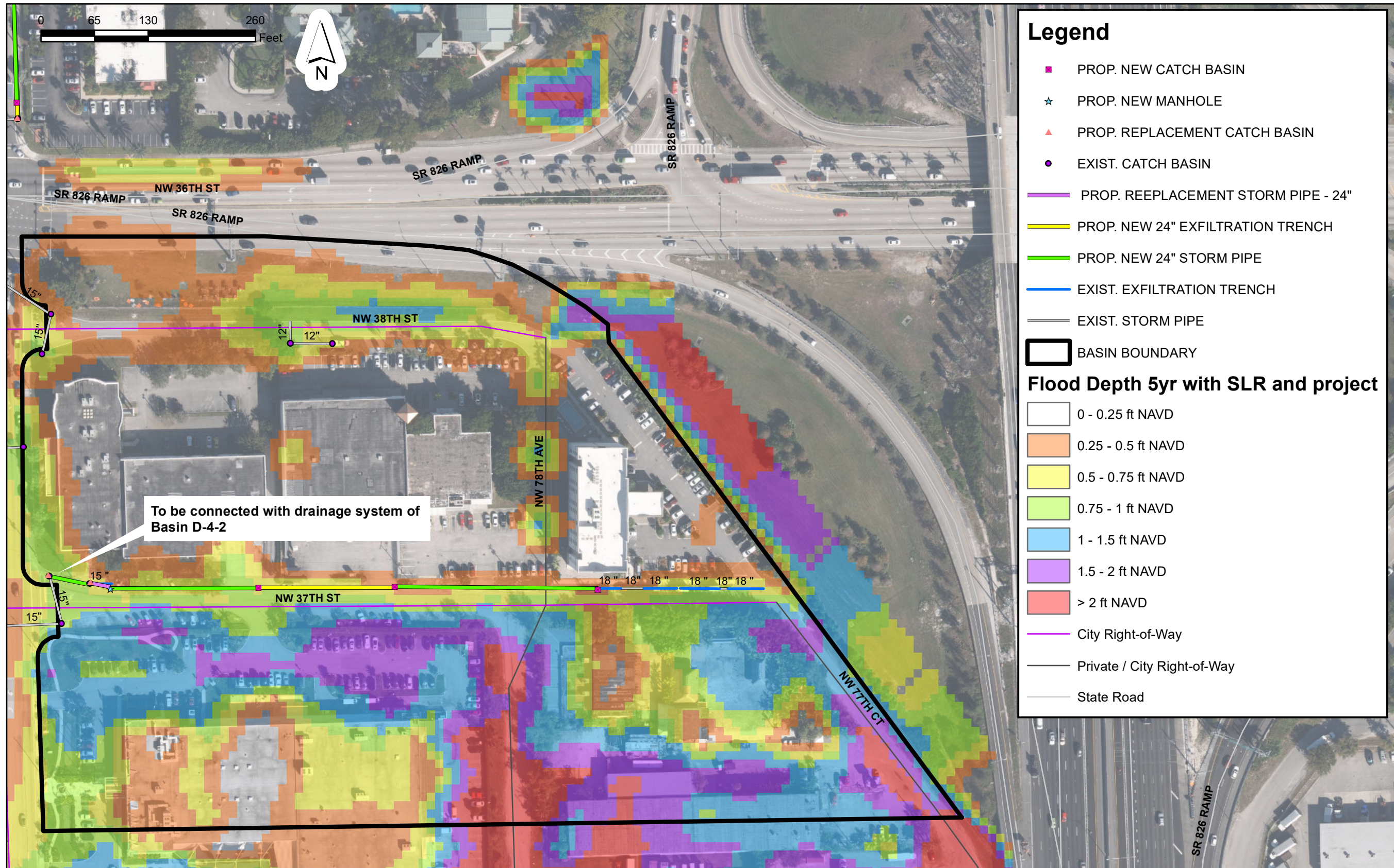
City of Doral Stormwater Management Master Plan Proposed Stormwater Projects Basin D-2-1 (Basin Rank 17) Cost Rank 4 - $204,138.38
