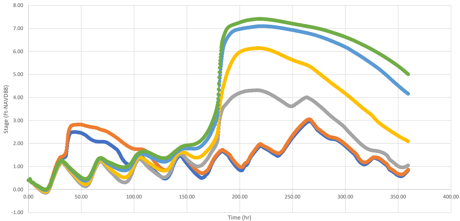
Time-Stage Hydrograph BD6 2020 - 25th Street Canal
