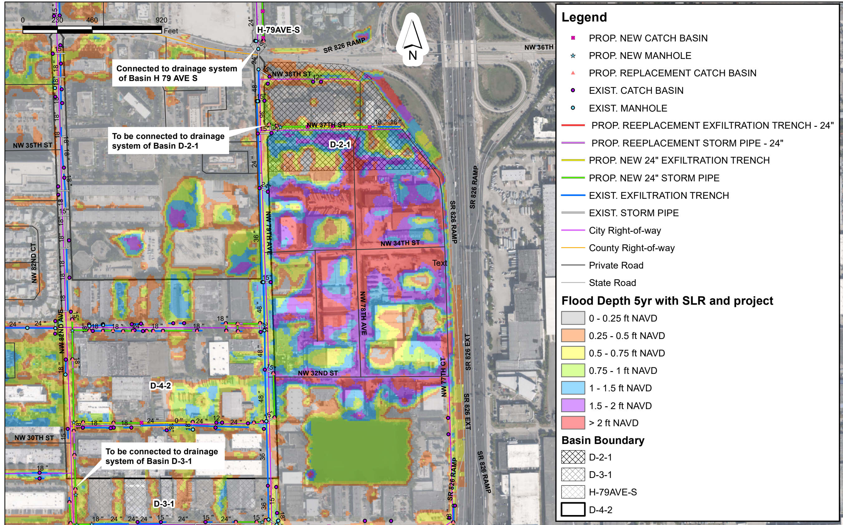
City of Doral Stormwater Management Master Plan Proposed Stormwater Projects Basin D-4-2 (Basin Rank 6) Cost Rank 5 - $937,994.33
