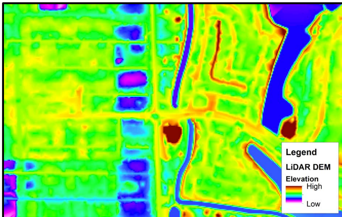
Figure 5-4 – LiDAR-based Raster DEM
