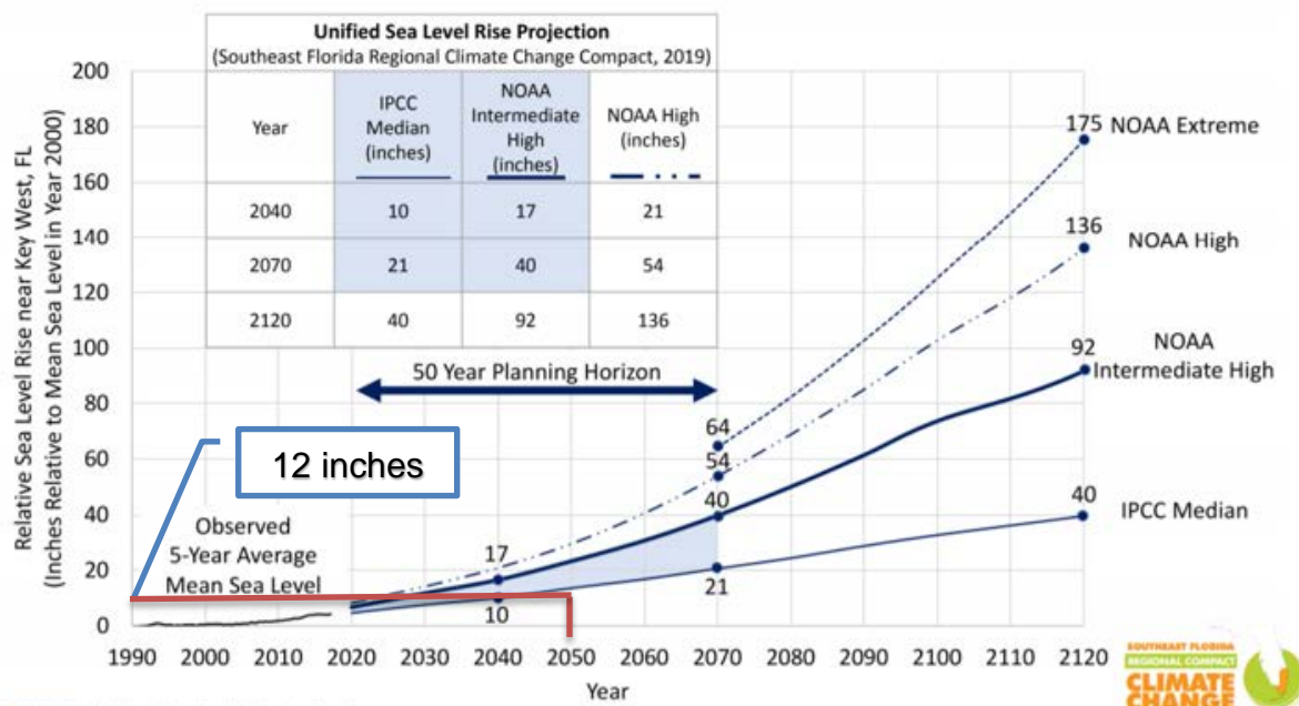
Figure 3-9 – Unified Sea Level Rise Projections for Southeast Florida (2019)
