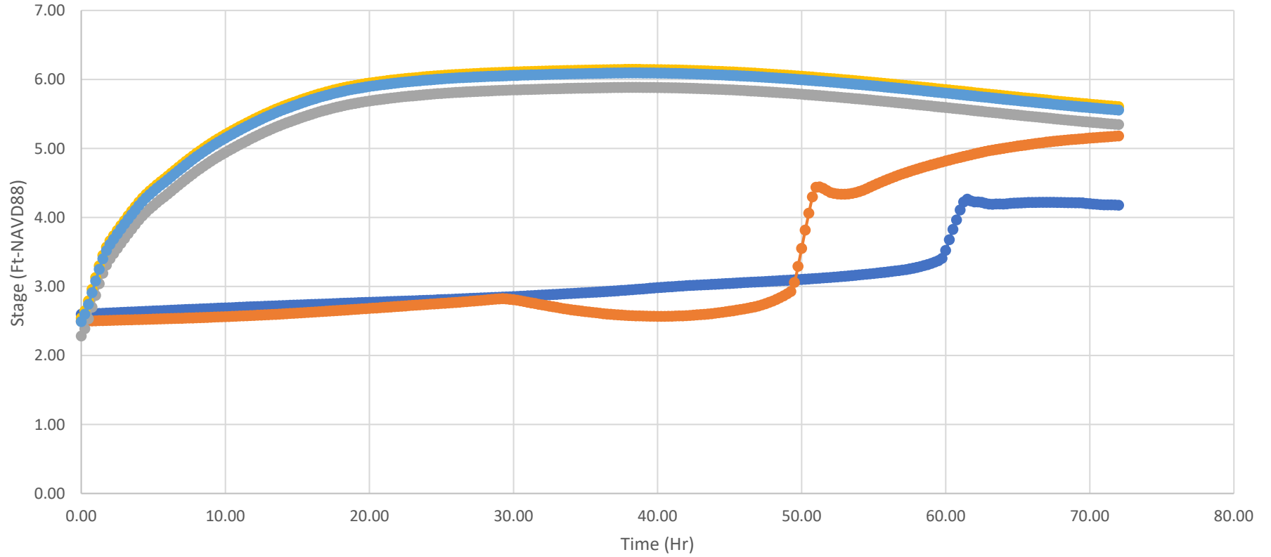
100YR-72HR TIME-STAGE HYDROGRAPH
