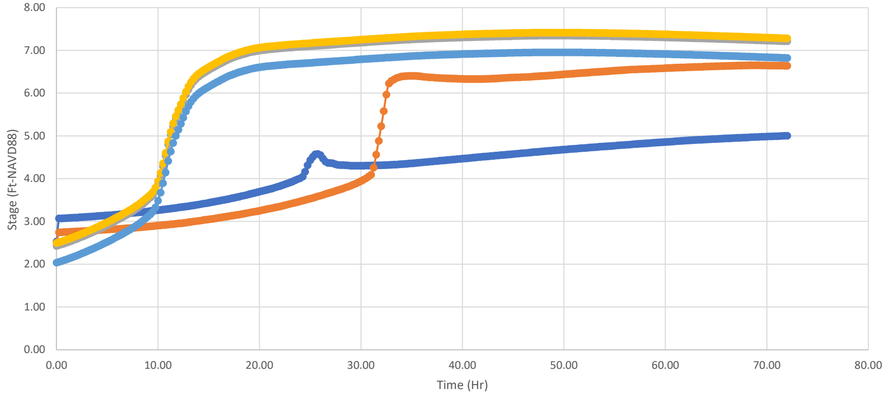
1000YR-72HR TIME-STAGE HYDROGRAPH
