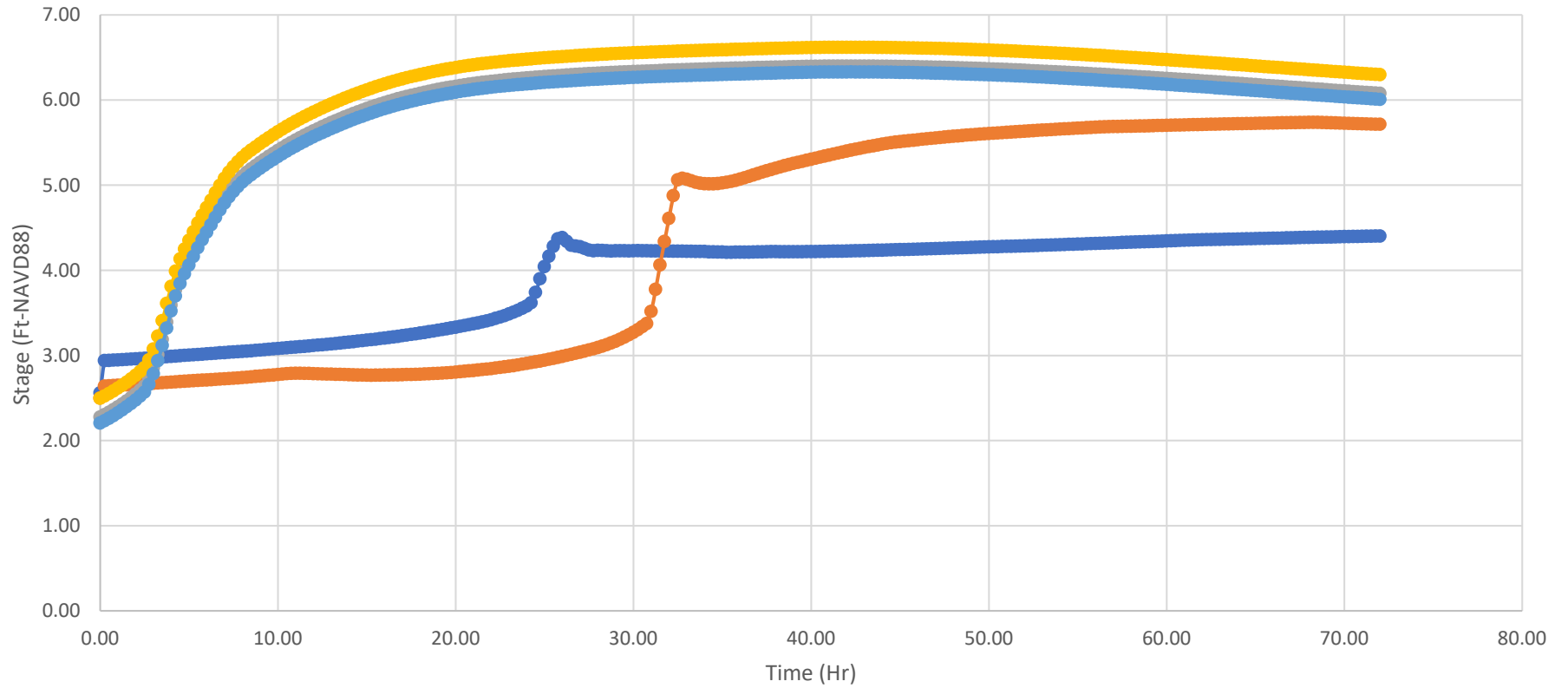
250YR-72HR TIME-STAGE HYDROGRAPH
