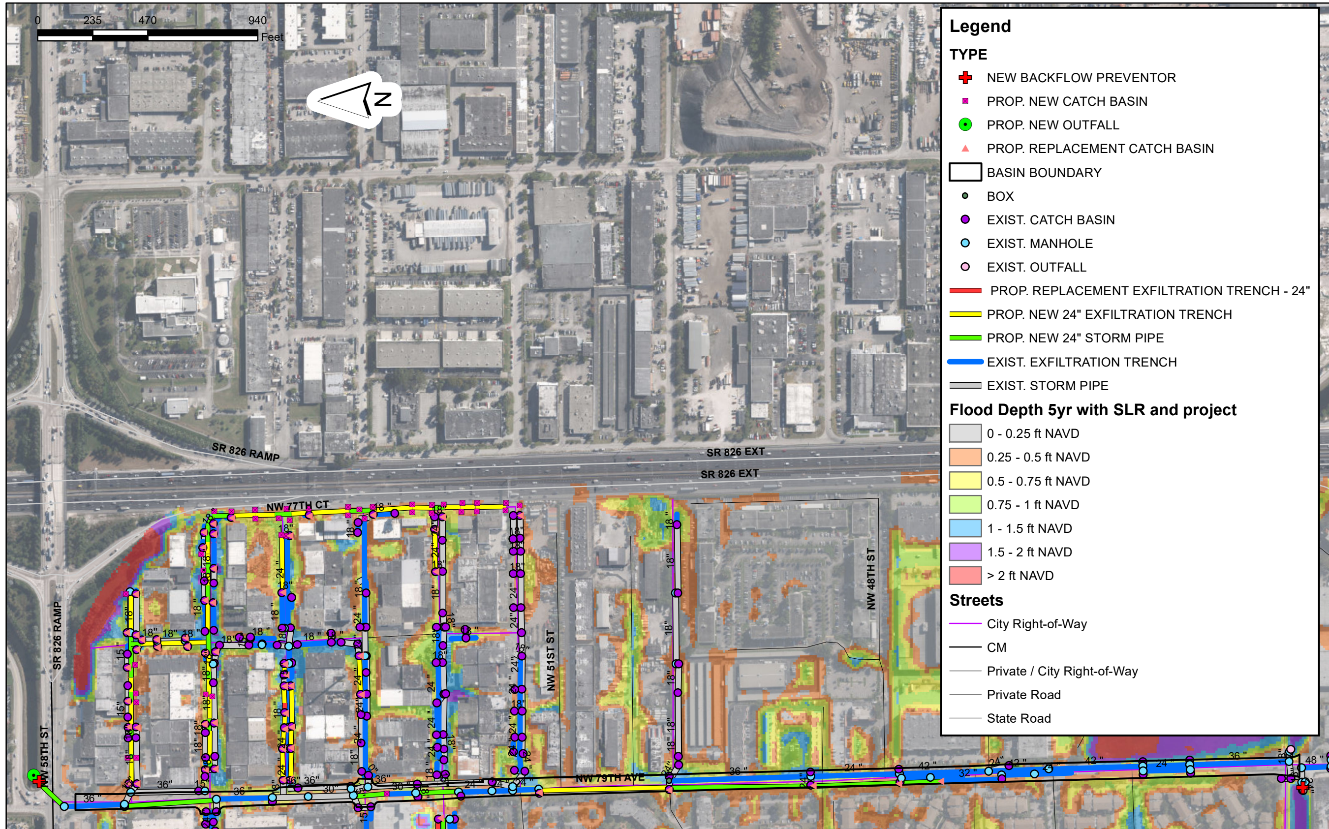
City of Doral Stormwater Management Master Plan Proposed Stormwater Projects Basin H-79AVE-N (Basin Rank 15) Cost Rank 17 - $417,610.88
