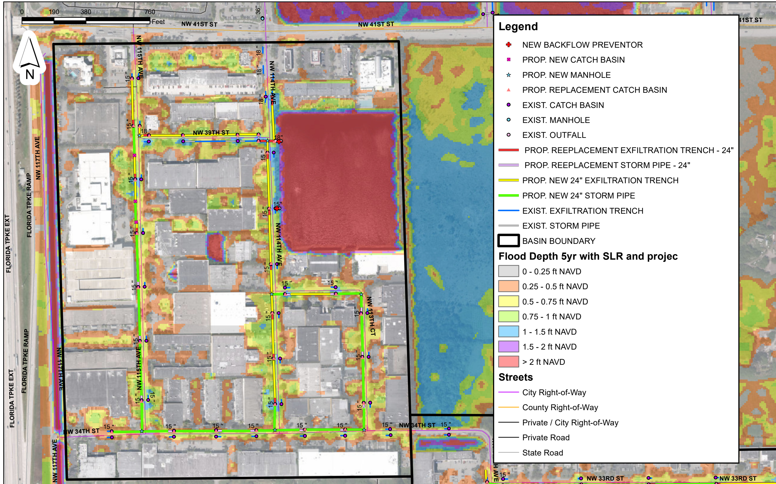
City of Doral Stormwater Management Master Plan Proposed Stormwater Projects Basin G4 (Basin Rank 13) Cost Rank 15 - $2,095,009.55
