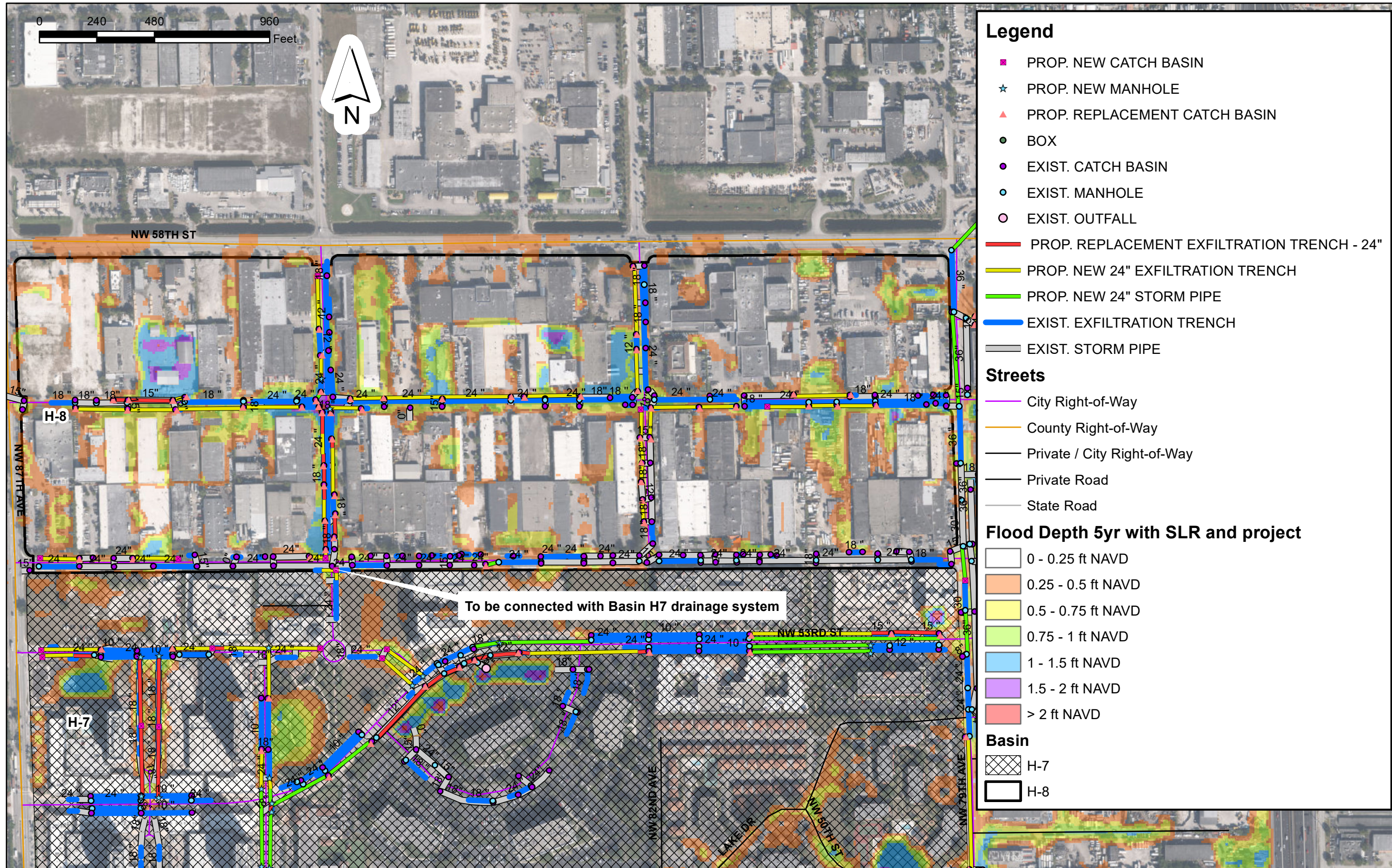
City of Doral Stormwater Management Master Plan Proposed Stormwater Projects Basin H8 (Basin Rank 4) Cost Rank 16 - $2,347,477.31
