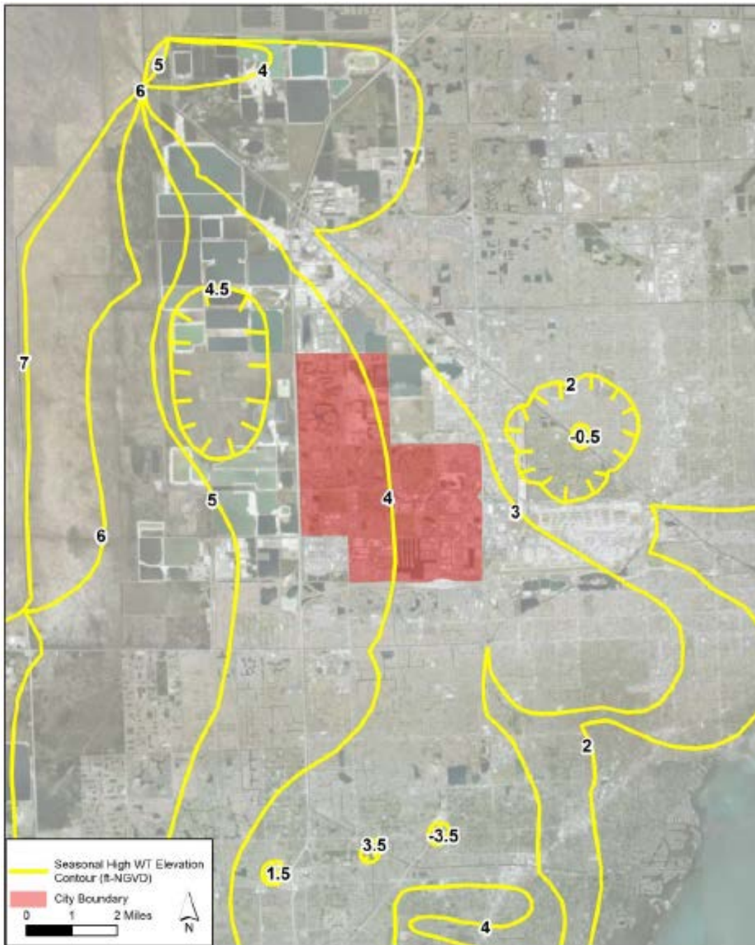
Figure 4-20 – Average October Groundwater Elevation
