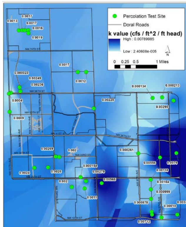
Figure 7-11 – Percolation Test Values and Locations
