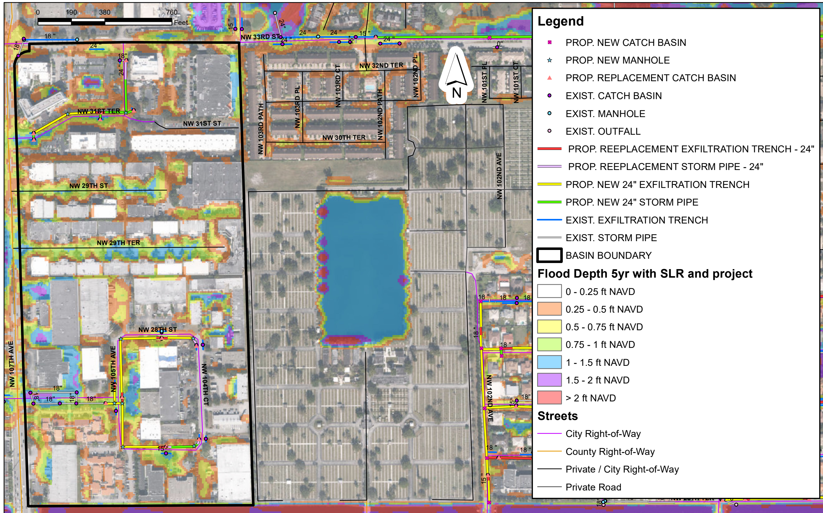
City of Doral Stormwater Management Master Plan Proposed Stormwater Projects Basin F5 (Basin Rank 10) Cost Rank 12 - $826,550.60
