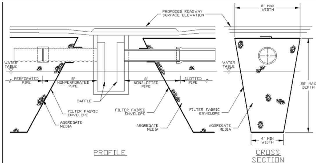
Figure 7-1 – Typical Exfiltration Trench Sections
