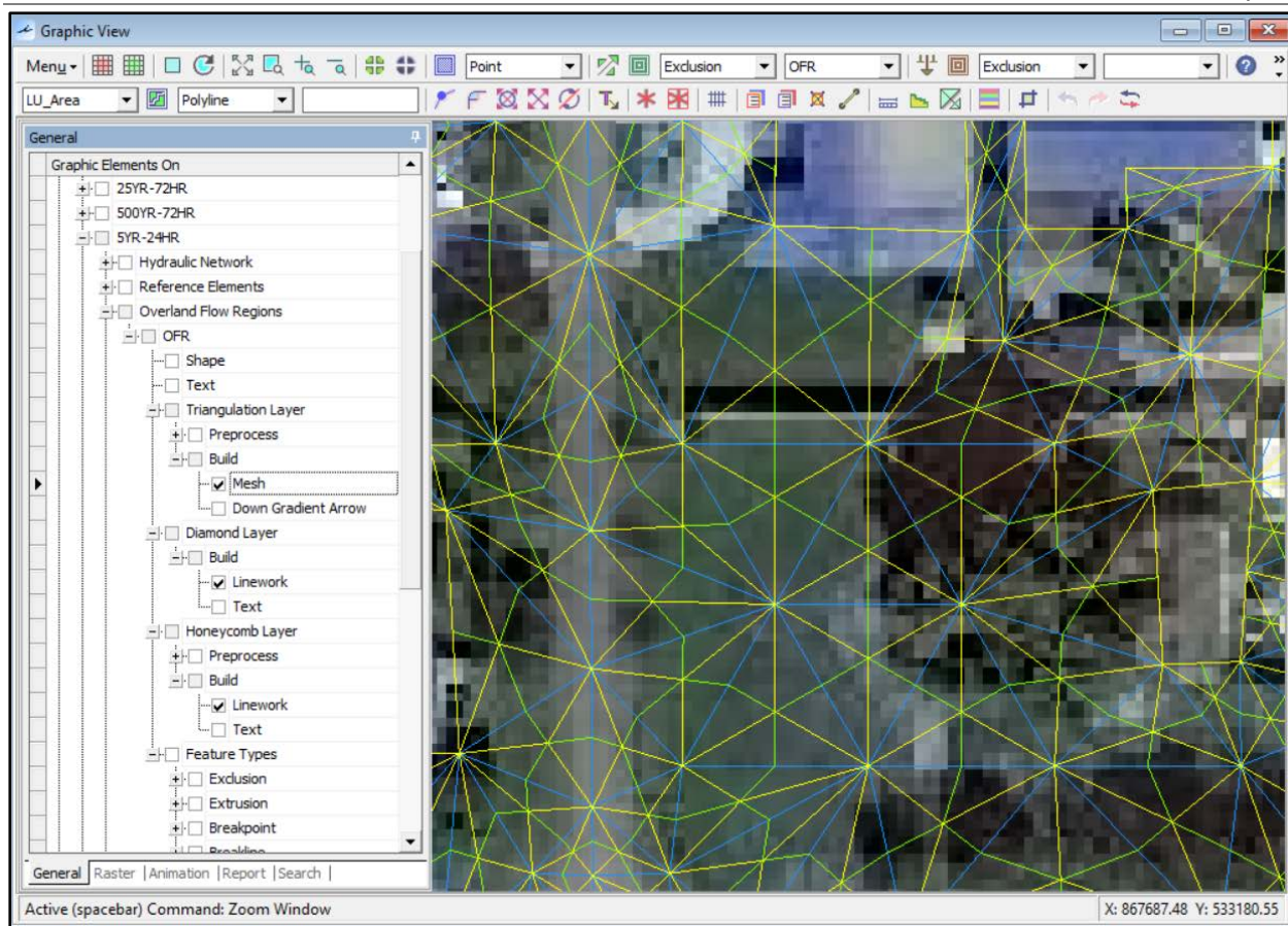
Figure 4-12 – Triangular, Diamond and Honeycomb Meshes
