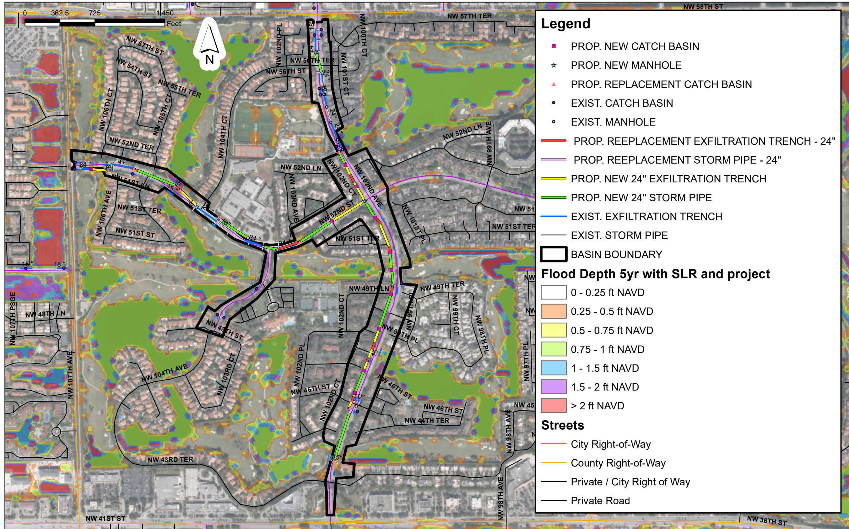
City of Doral Stormwater Management Master Plan Proposed Stormwater Projects Basin NW 52 ST W (Basin Rank 11) Cost Rank 13 - $1,488,362.73
