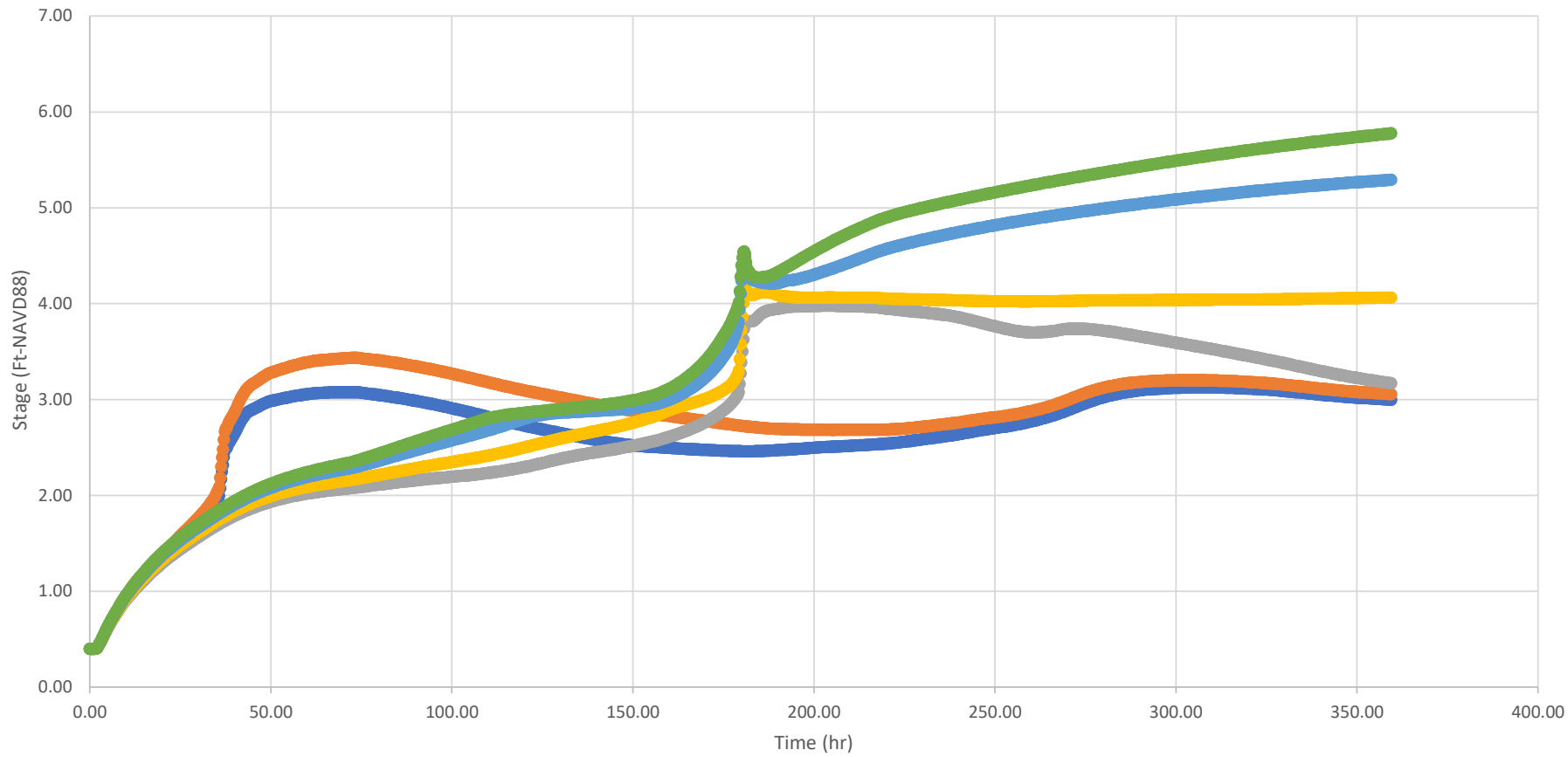
Time-Stage Hydrograph BD1 2020 - Snapper Creek North
