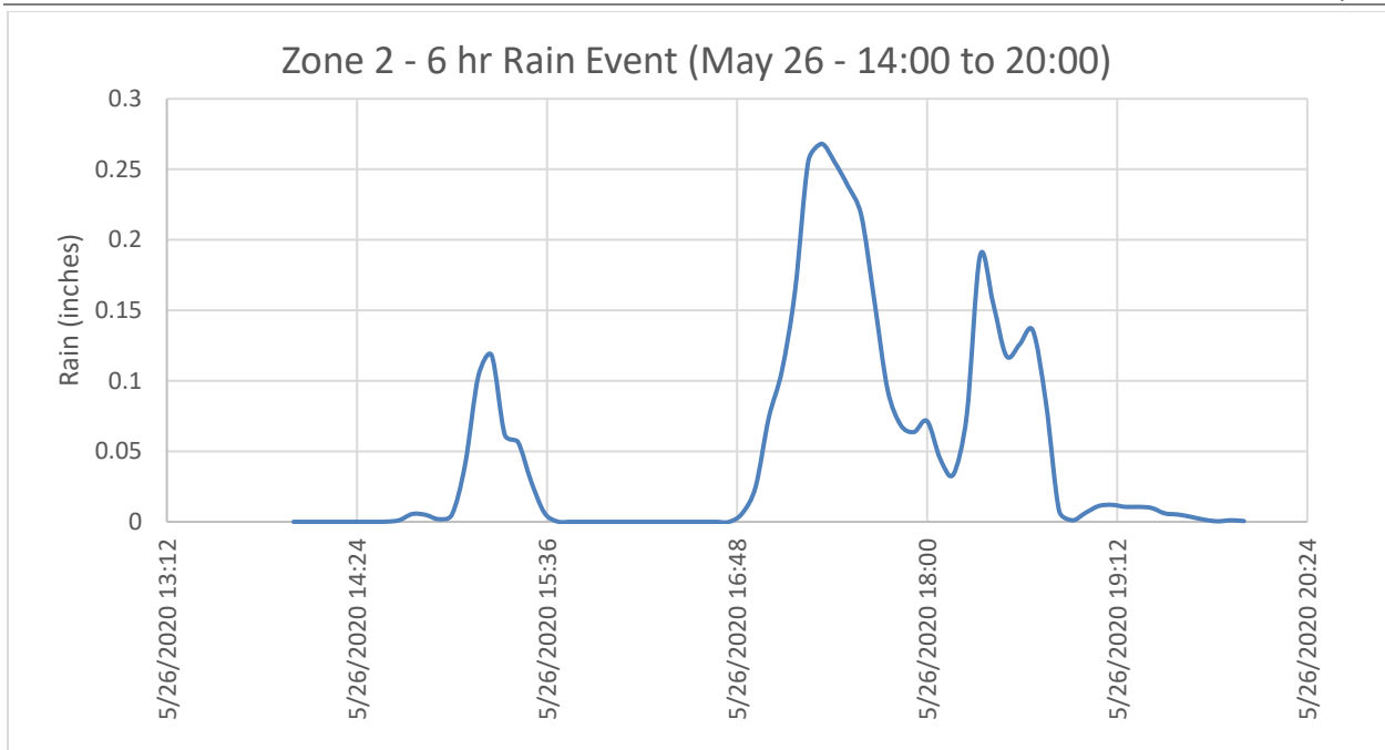
Figure 4-17 – Rain Zone 2 Hydrograph
