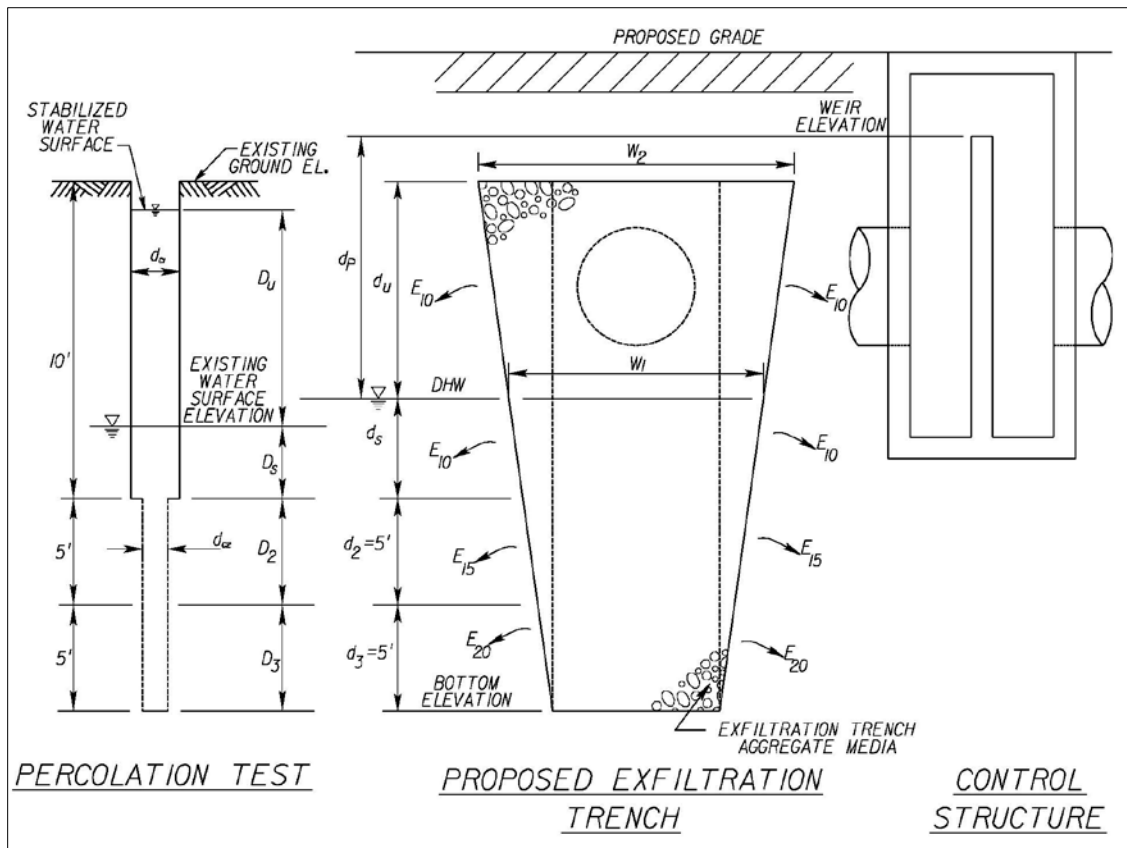
Figure 7-2 – Schematic of the percolation test parameters compared to the proposed exfiltration trench and control structure. Condition where DHW is within the trench aggregate media and the control elevation is above the trench aggregate media.
