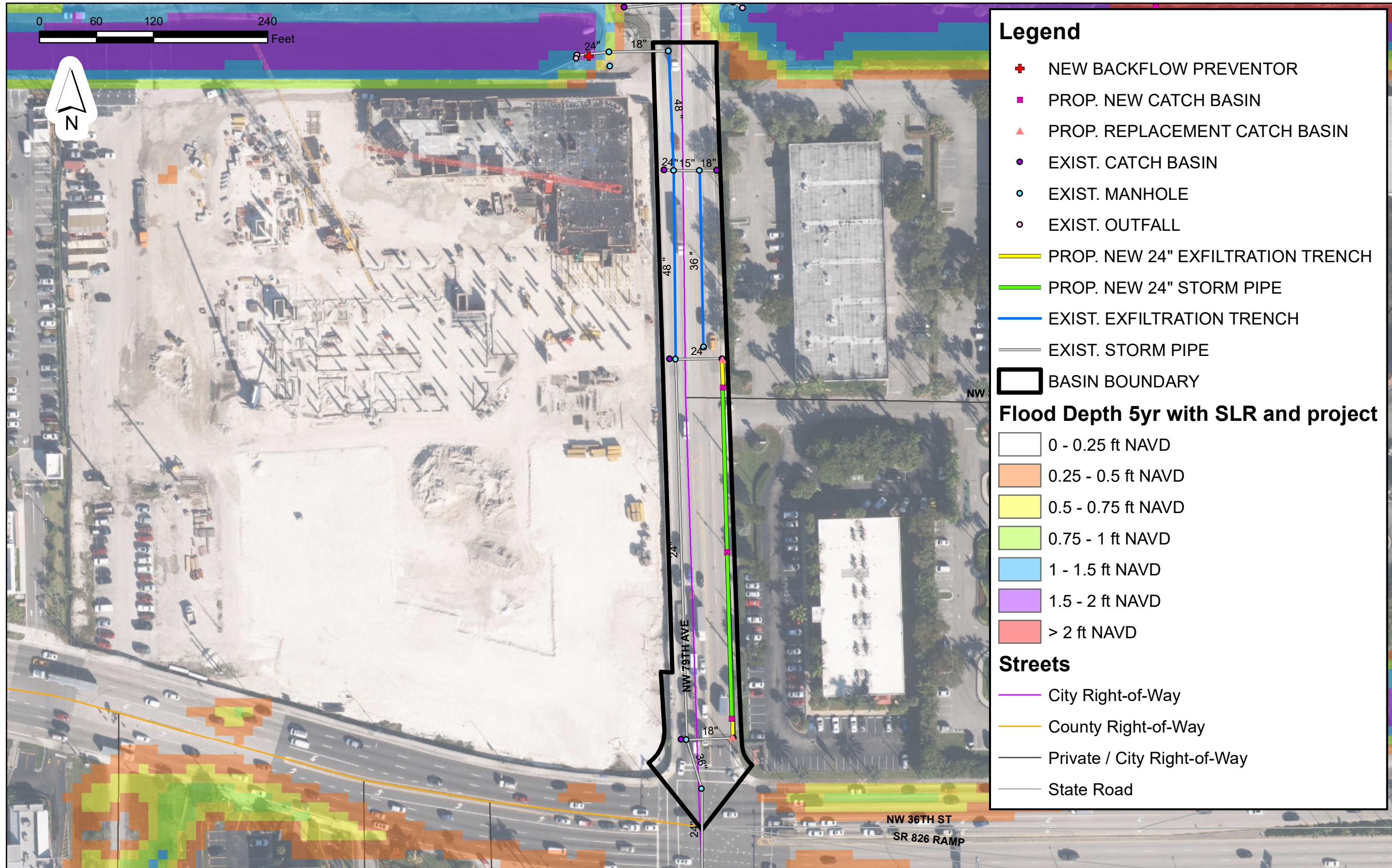
City of Doral Stormwater Management Master Plan Proposed Stormwater Projects Basin H 79 AVE S (Basin Rank 16) Cost Rank - $253,849.67
