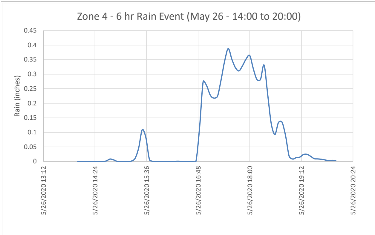
Figure 4-19 – Rain Zone 4 Hydrograph
