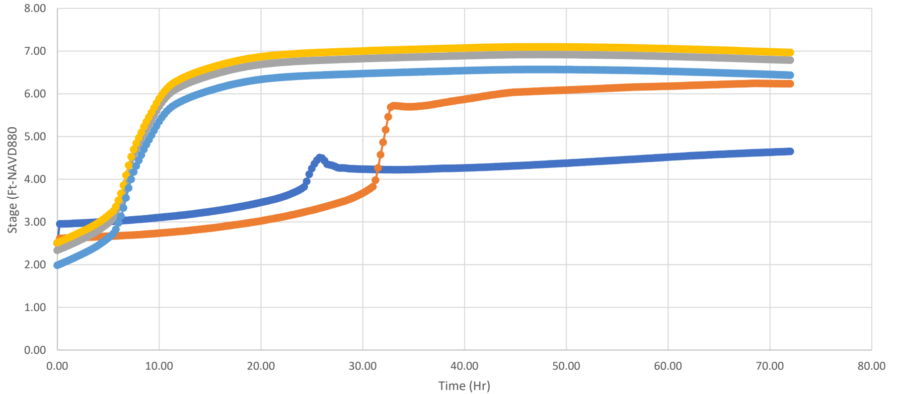
500YR-72HR TIME-STAGE HYDROGRAPH
