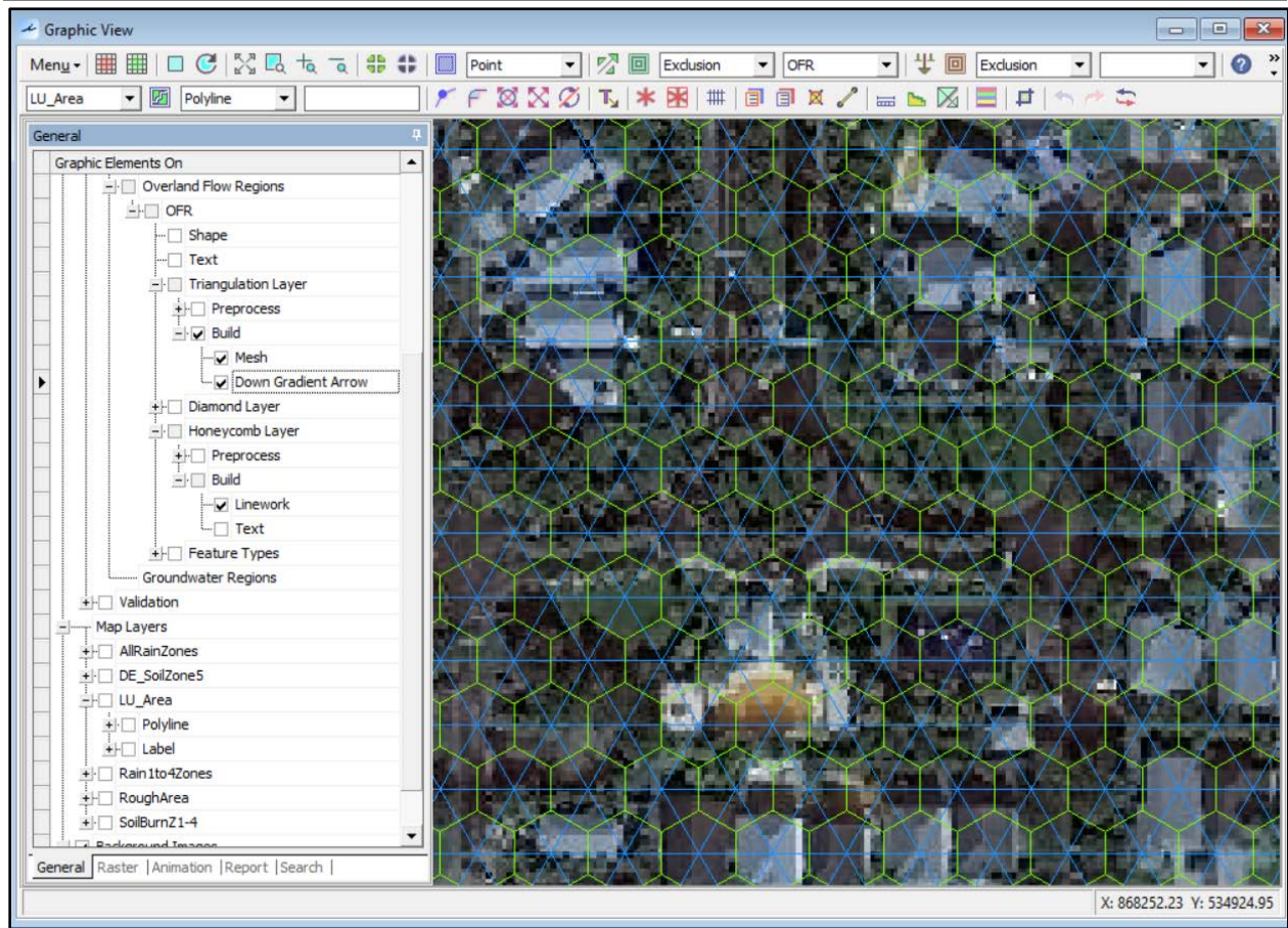
Figure 4-10 – Mesh and Honeycomb for a Section of the City’s Domain
