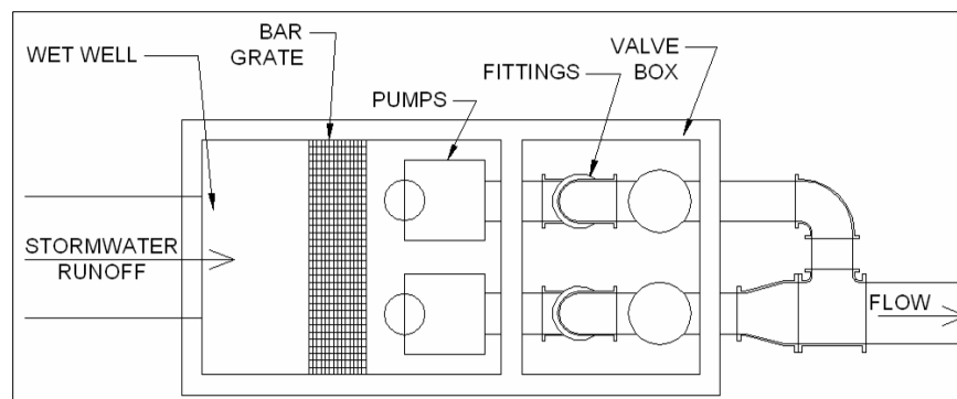
Figure 7-5 – Typical Stormwater Pump Station Plan View
