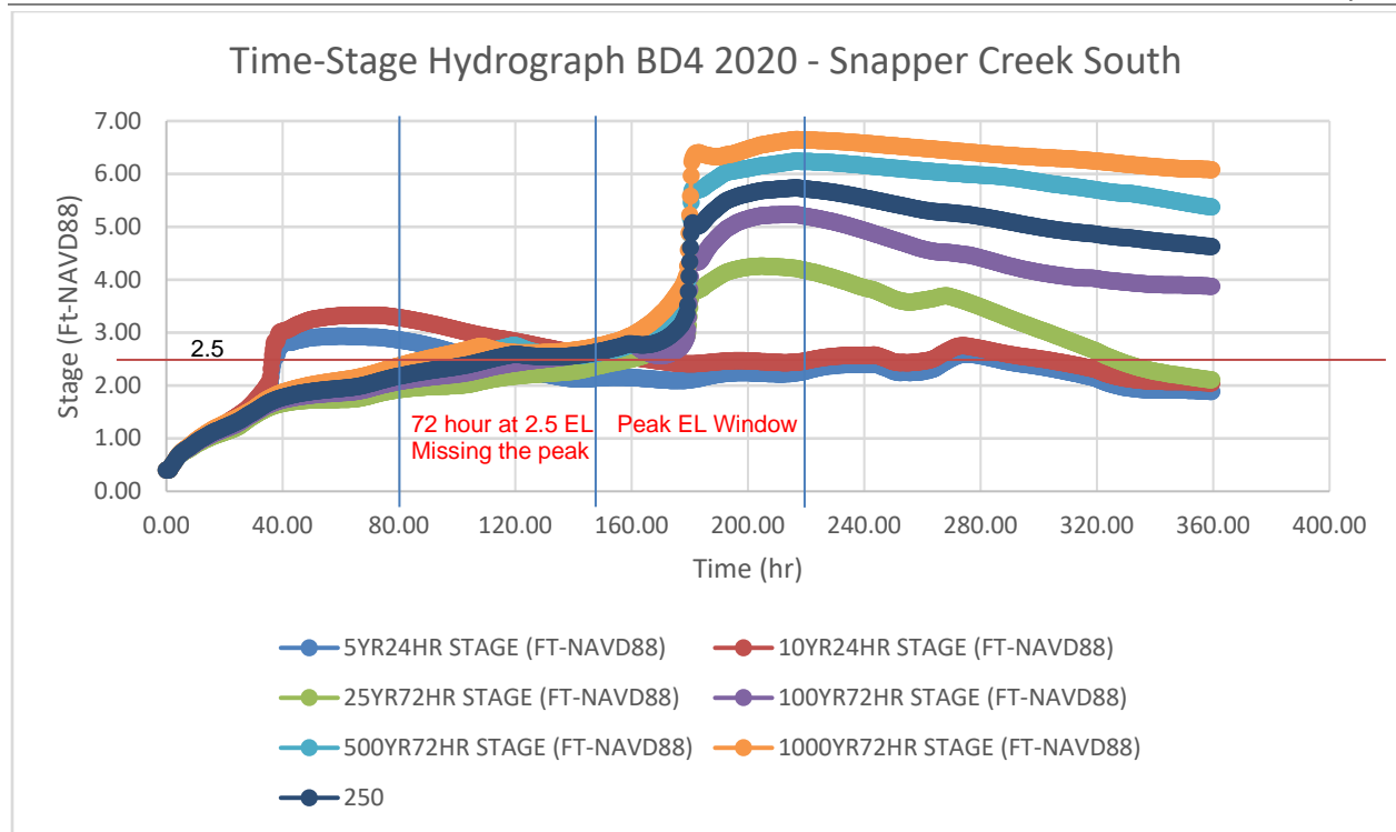
Figure 4-21 – Time-Stage Hydrograph for BD4
