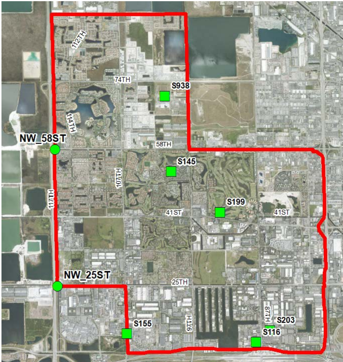
Figure 3-1 – Map of Rain Gauges and Canal Points in the City of Doral
