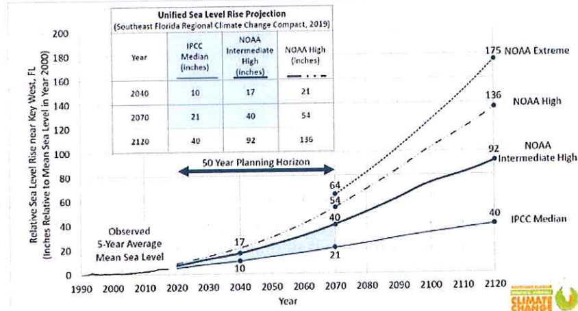
Figure 6-1: Southeast Florida Regional Climate Compact SLR Projections
