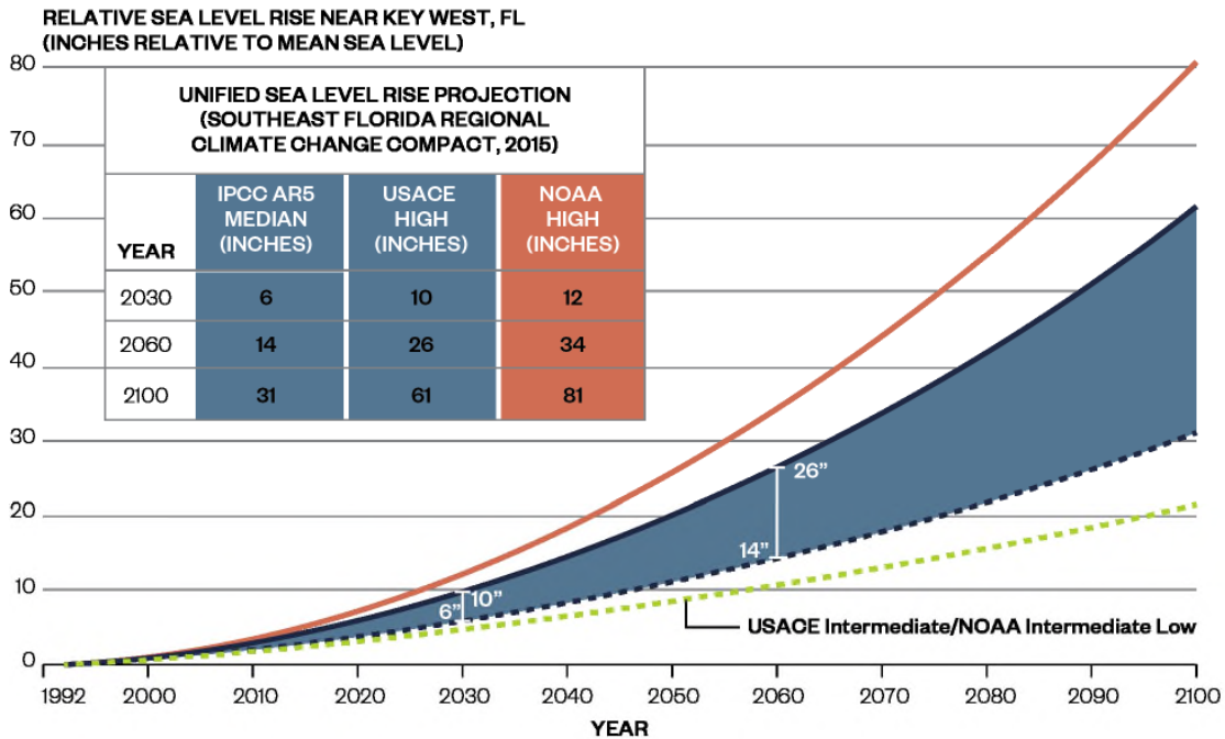
Figure 5-1 – Sea Level Rise Projection (Southeast Florida Regional Climate Change Compact, 2015)
