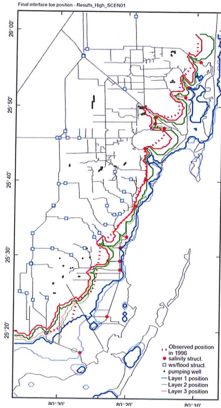
Figure 6-4: Scenario 3 Salt Water Intrusion Results. (Walsh and Hughes, 2014).
