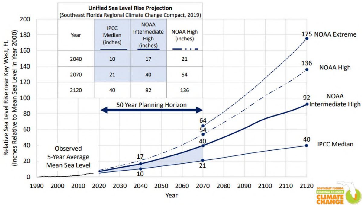
Figure 5-2 – Sea Level Rise Projection (Southeast Florida Regional Climate Change Compact, 2019)
