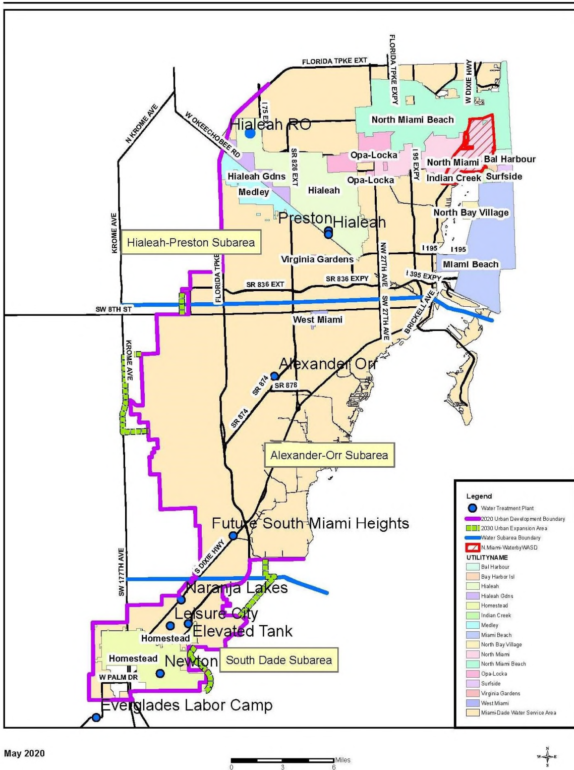
May 2020 Figure 3-2: WSD Subareas, Water Treatment Plants, and Wholesale Water Customers (From: Miami-Dade County Water and Sewer Department, 2020)
